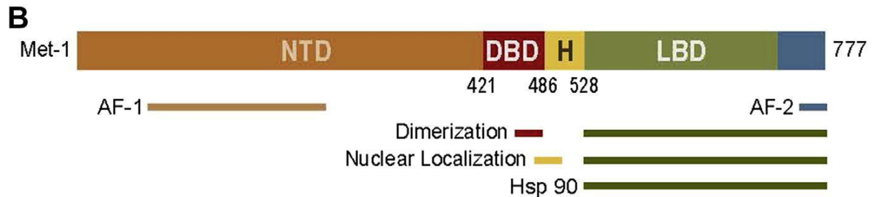
Figure 1. Glucocorticoid receptor
